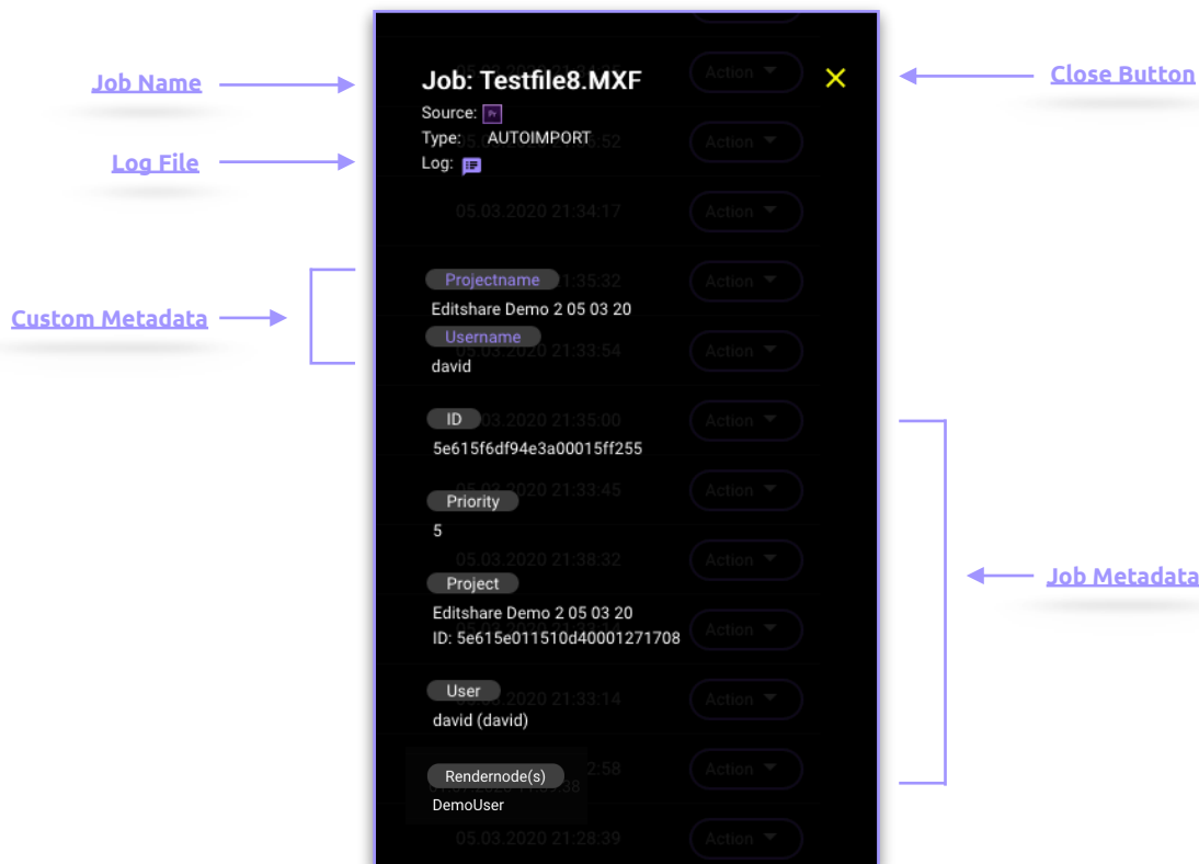
Figure 2.4.4 Hidden Overlay
