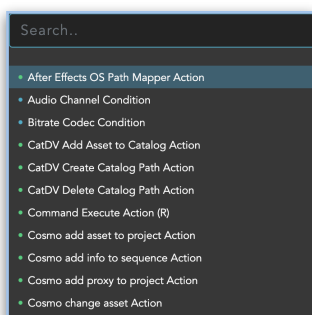
Figure 2.7.1 Mode 1
