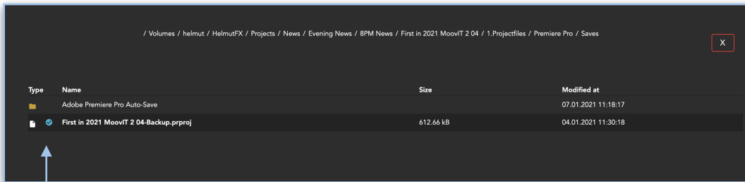
Figure 2.4.4. File Chooser
