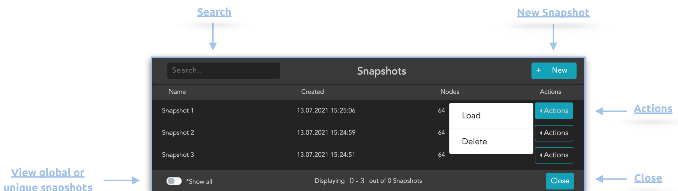
Figure 2.3.2. Snapshots
